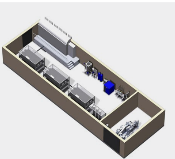
Figure 2. 1 MW Turnkey Electrolyser (Hydrogenics).
